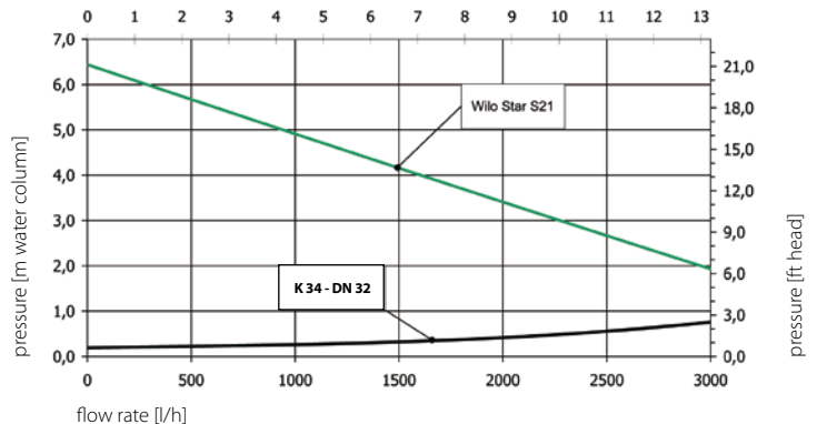
Pressure drop K34 / pump characteristics flow rate [USgpm]
