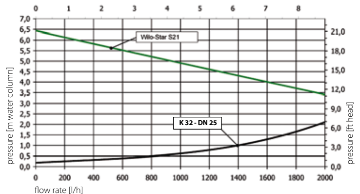
Pressure drop K32 / pump characteristics flow rate [USgpm]
