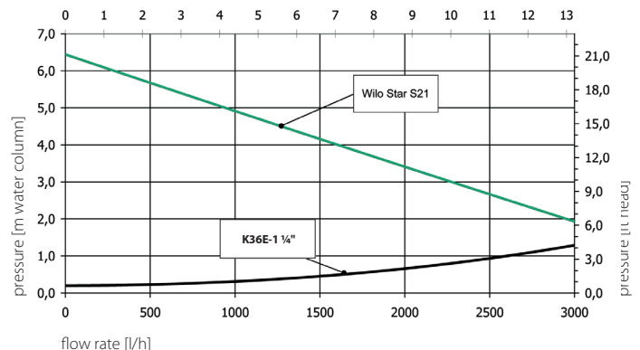
Pressure drop K36E/pump characteristics flow rate [USgpm]
