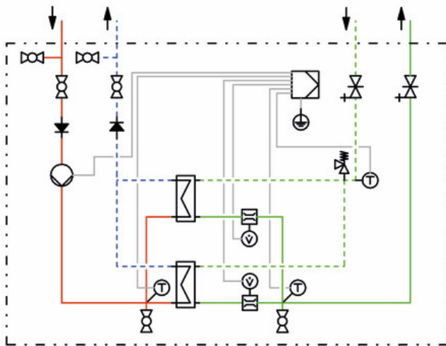
Domestic hot water module without circulation
