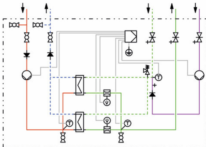
Domestic hot water module with circulation
