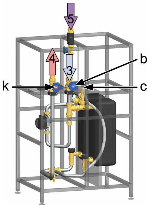
Secondary circuit
