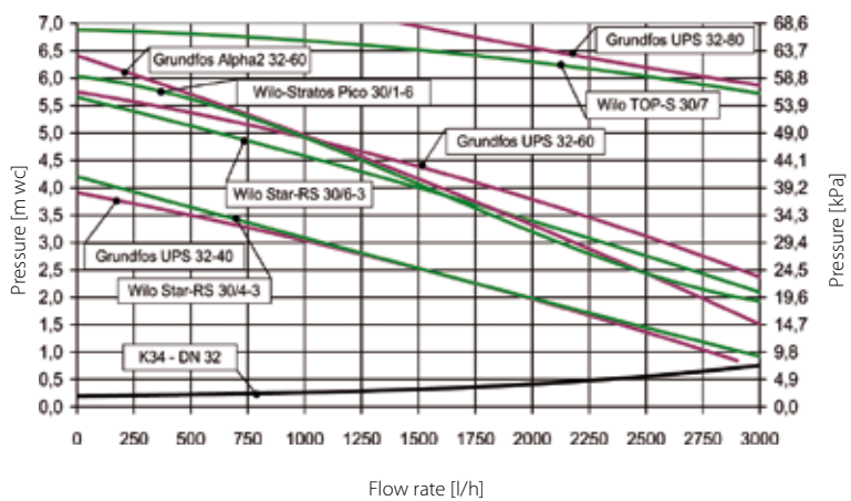
Differential pressure diagram K34
