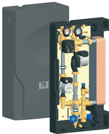
Tank heat transfer module
